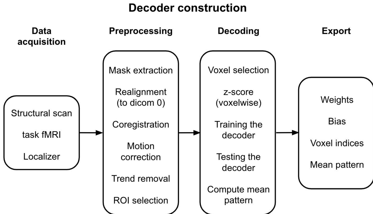
Figure 3. General steps included in decoder construction. In order to conduct decoder construction, a structural scan as well as functional data from an fMRI task typically need to be acquired for each participant. A functional localizer session can also be included at this stage in order to functionally select the voxels to be used in the decoding procedure. The preprocessing steps follow standard fMRI procedure with a specific consideration for conducting steps that will also be possible to conduct online. Afterwards, the decoding steps will aim to determine the accuracy of the decoder. Once the decoder has been trained, it is important to export all the information that will be required to conduct the online decoding procedure.
